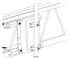
Truss (Purlin) Installation
